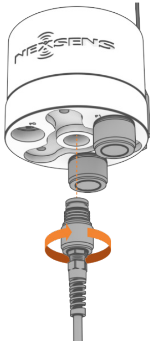
Figure 2: UW-6 Plug connection to an X2 data logger power port.
