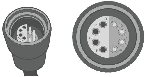
Figure 3: UW Receptacle pinout.
