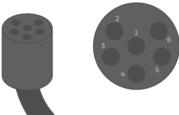
Figure 2: MCIL-6 female style pinout.
