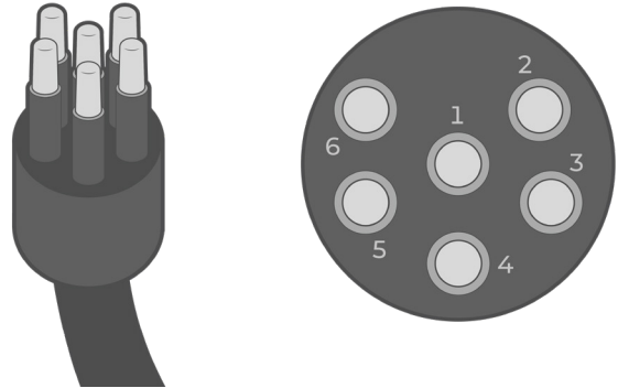
Figure 3: MCIL-6 male style pinout.
