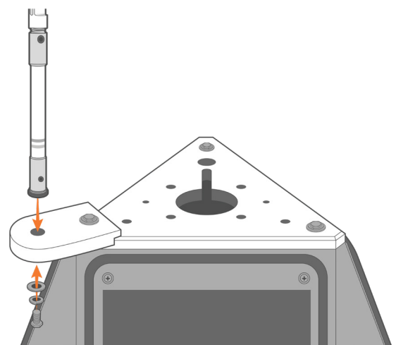
Figure 4: Install a top-side instrument mount.
