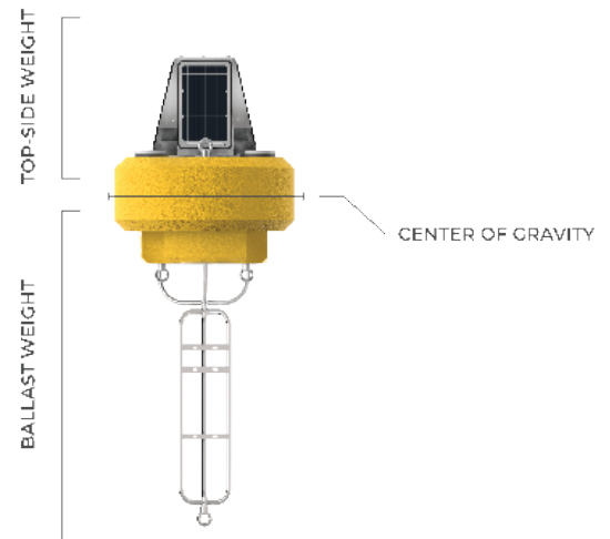
Figure 6: CB-450 buoyancy diagram.
