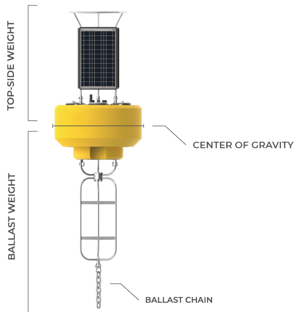
Figure 5: CB-1250 buoyancy diagram.
